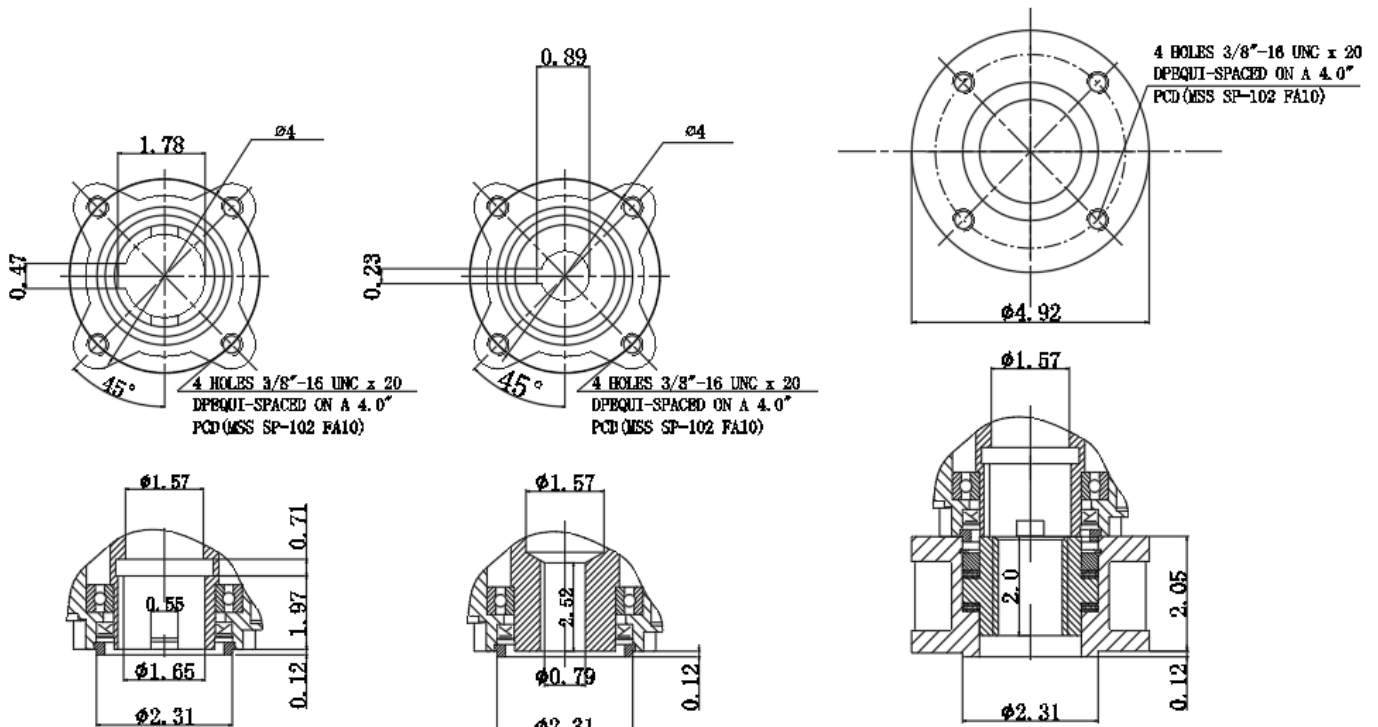
FA10 flange B1 interface
