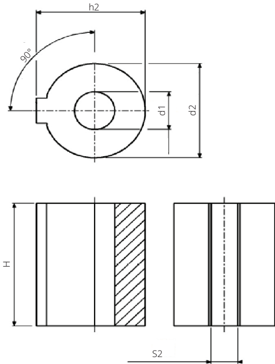
Figure 13. Unmachined Insert (Special Key) Dimensions
