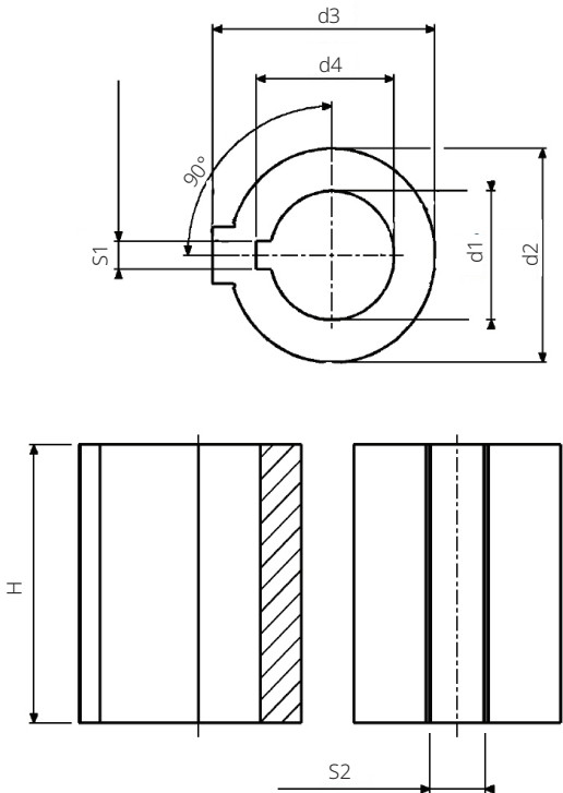
Figure 12. Keyed (Special Key) Dimensions
