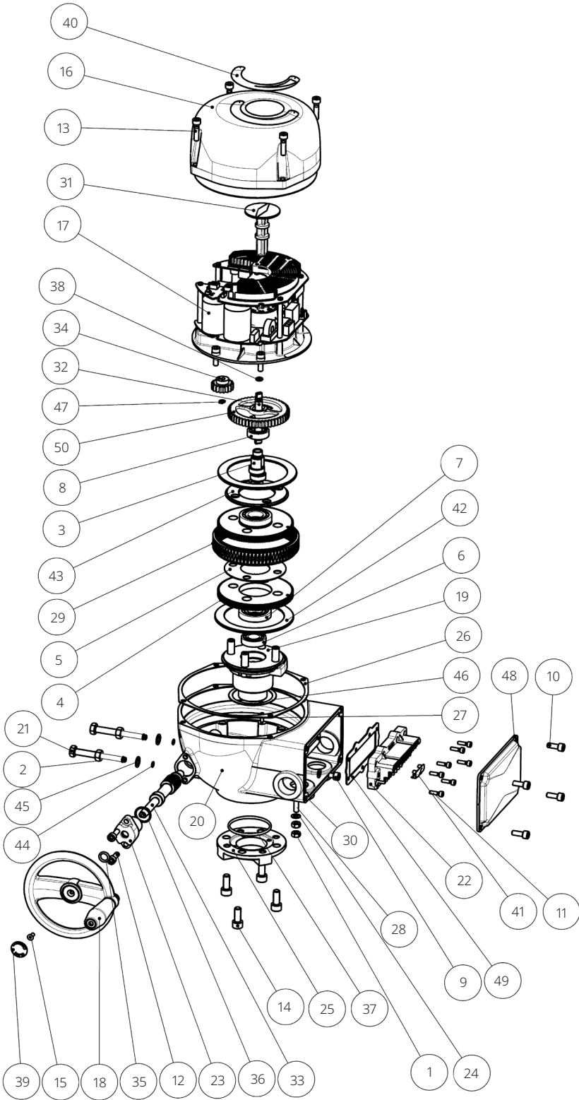
Figure 1. Component Parts for Models 063 / 125 / 250/ 500 / 1000
