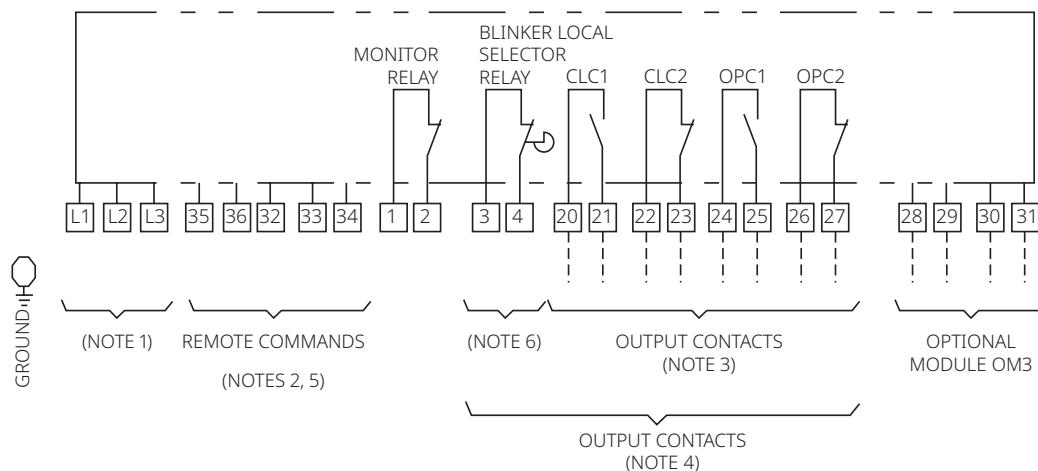
Figure 14. SCE300 Wiring Diagram
