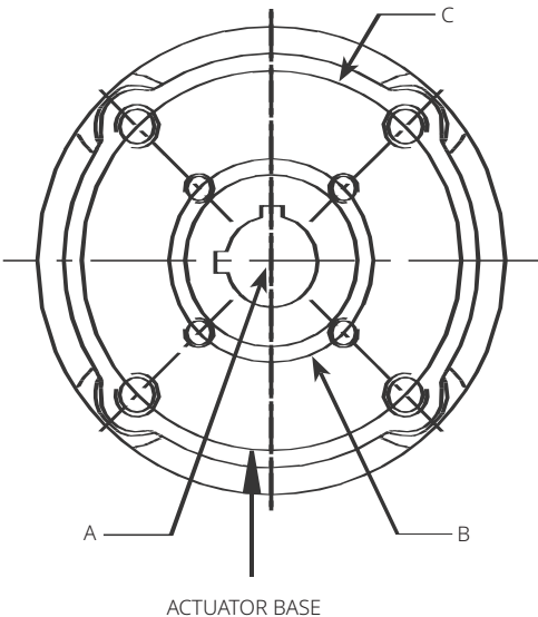
Figure 7. Actuator Drive Insert and Bolt Circles
