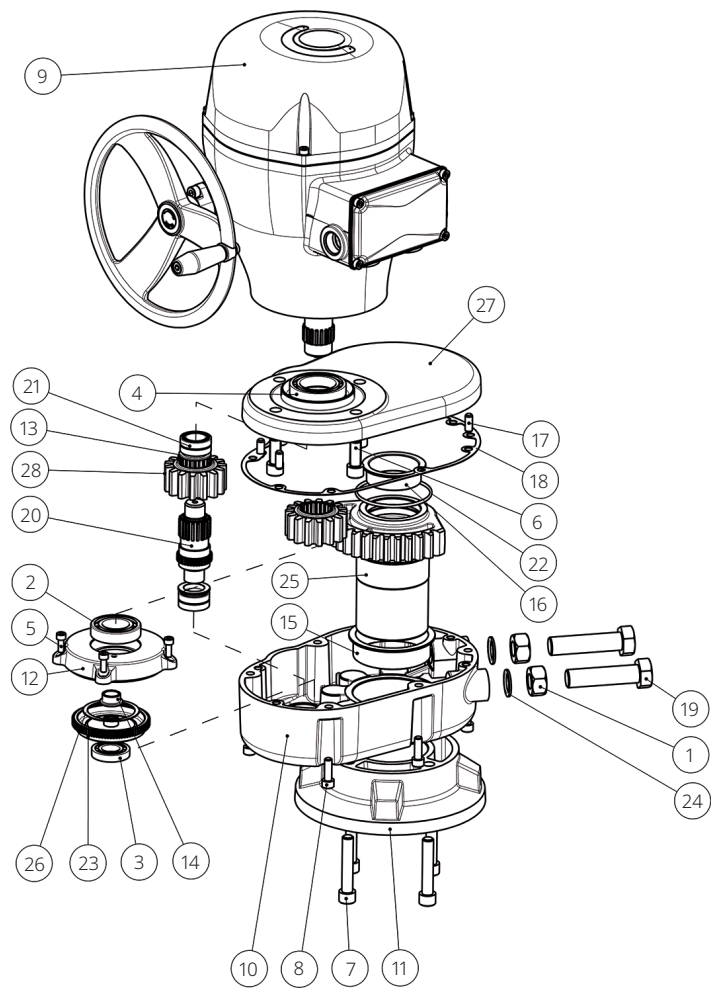
Figure 2. Component Parts for Model 200
