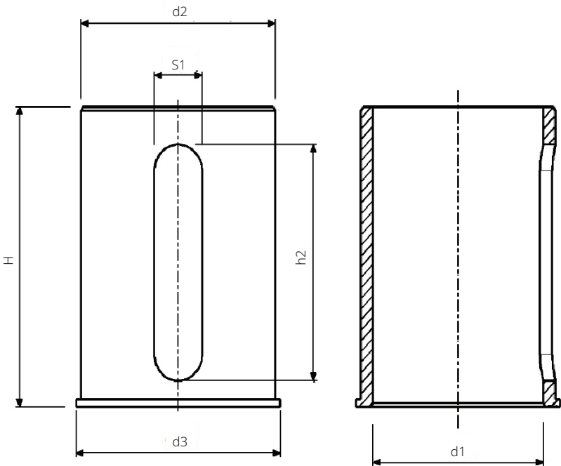
Figure 11. Keyed (Special Key) Dimensions
