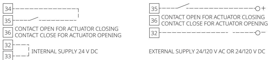
Figure 15b. Two Wires Setting (to be Configured)
