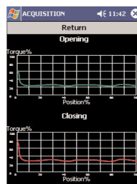
Valve torque curve for preventative maintenance
